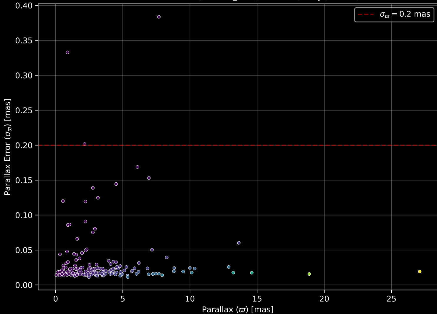
APOGEE DR17 Field: [177+34_MGA] Parallax Quality (n= 188)
