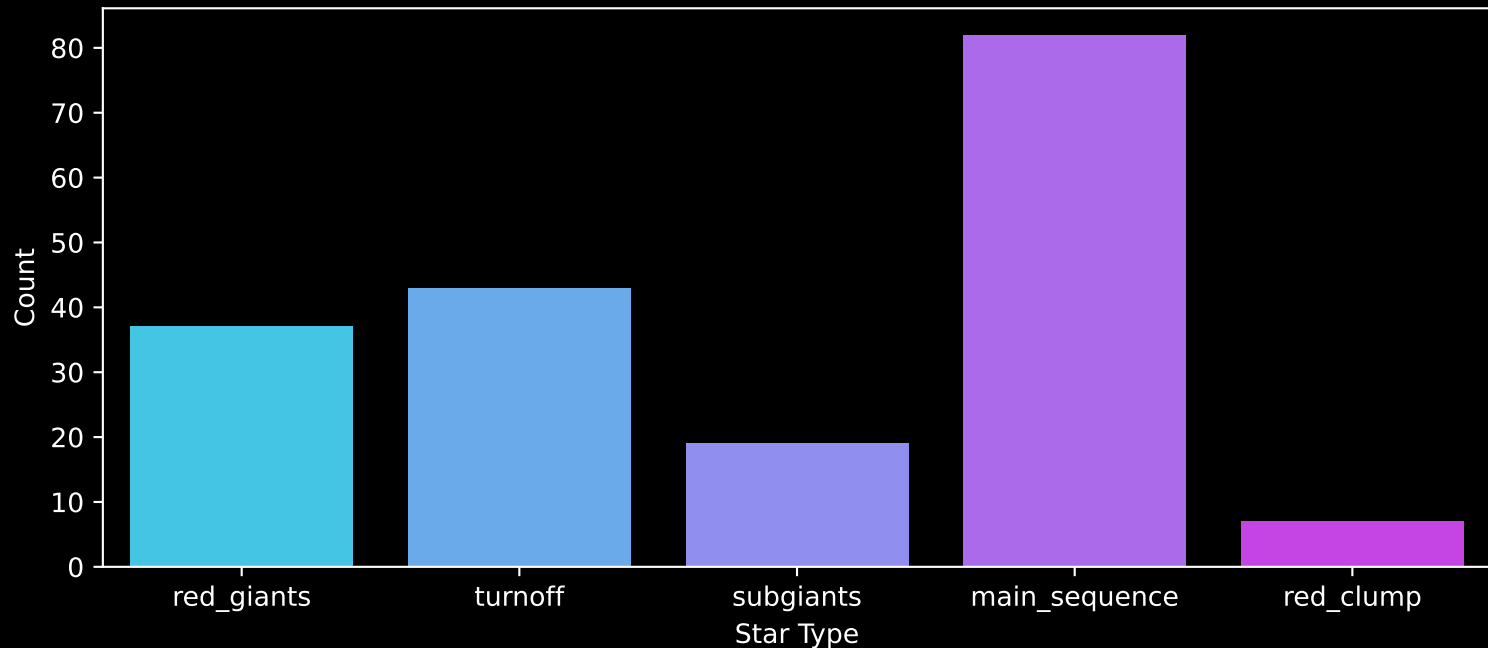
APOGEE DR17 Field: [177+34_MGA] Count plot of Star Type
