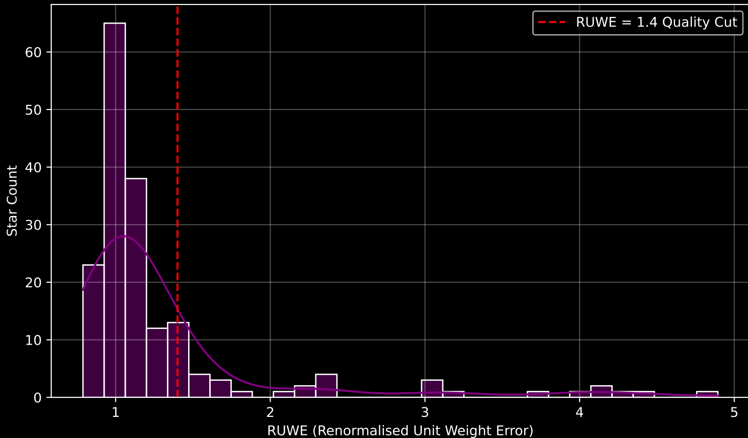
GAPOGEE DR17 Field [177+34_MGA] RUWE Distribution (n= 177)
