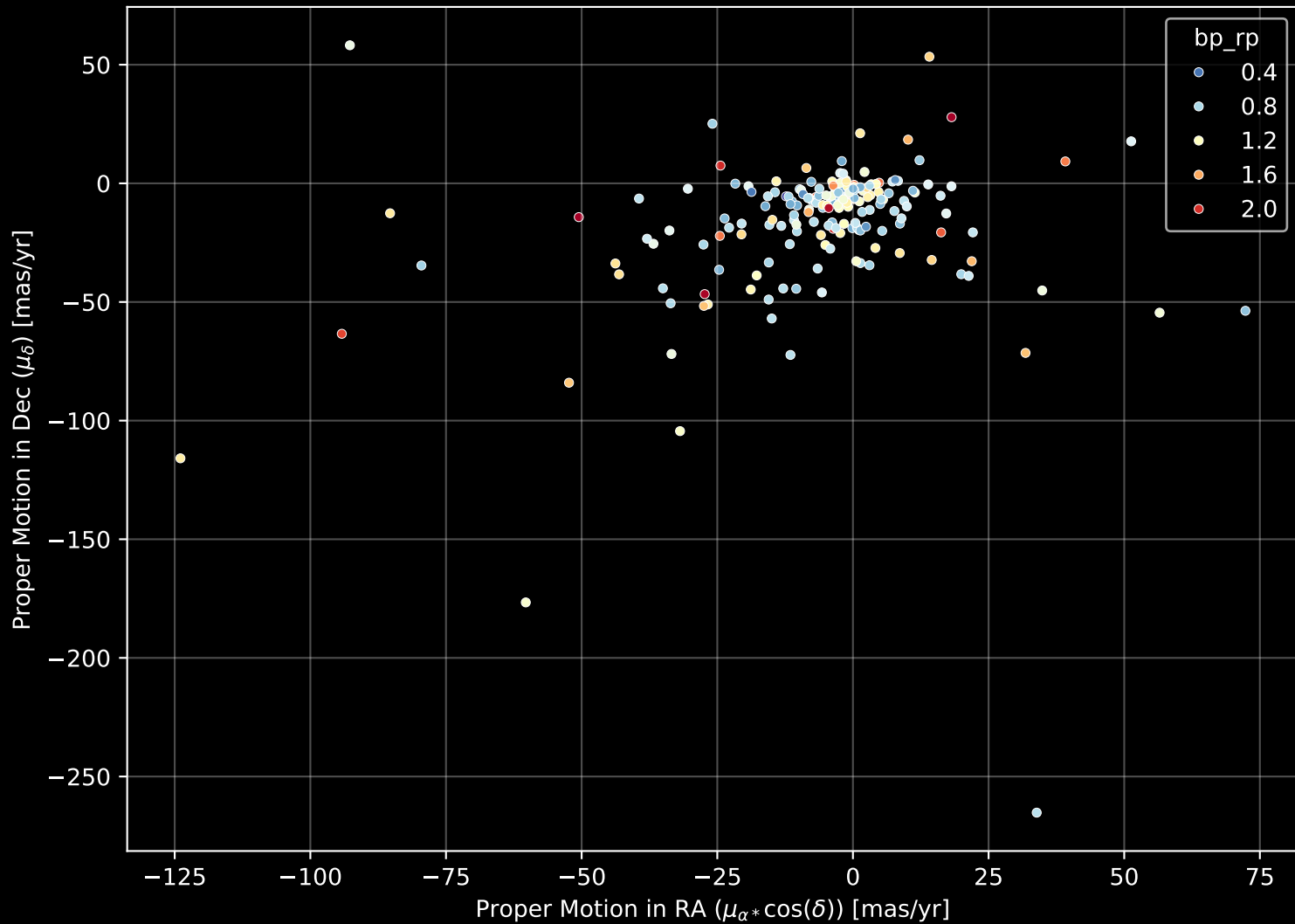
APOGEE DR17 Field: [177+34_MGA] Proper Motion Diagram (n= 188)
