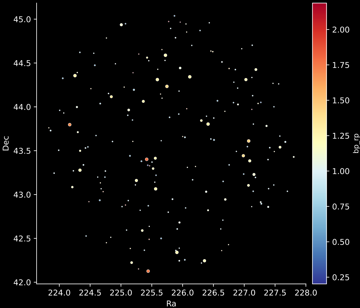
APOGEE DR17 Field: [177+34_MGA] Stars: 188
