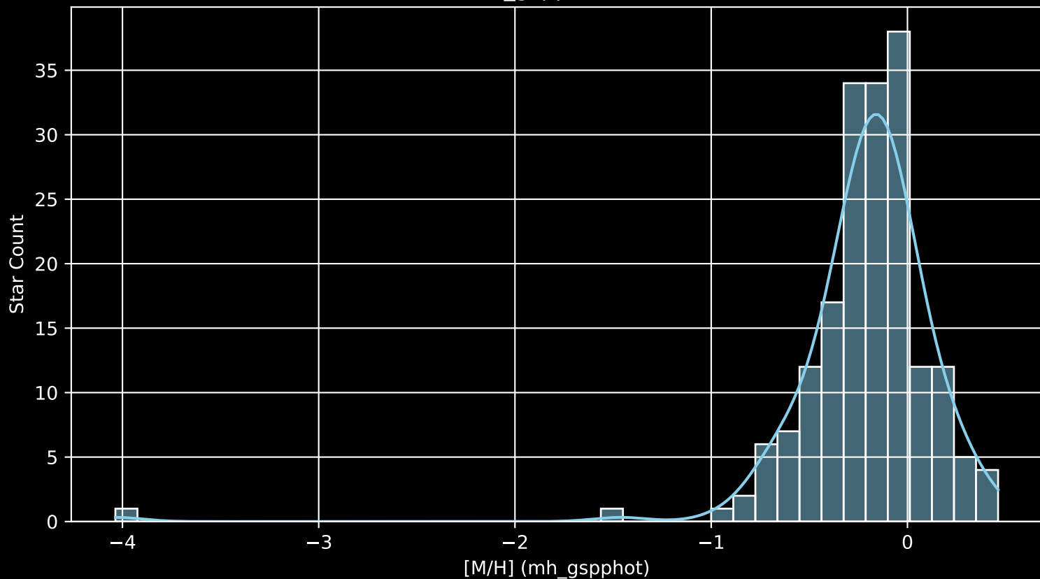
APOGEE DR17 Field: [177+34_MGA [M/H] (mh_gspphot) (n= 186)
