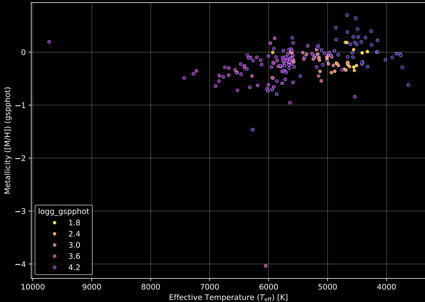
APOGEE DR17 Field: [177+34_MGA] Stellar Population Parameters (n= 188)
